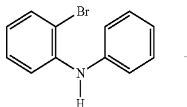
[Reaction Scheme 7]
