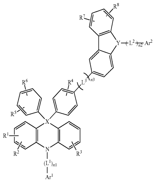
[Chemical Formula 1-4]
