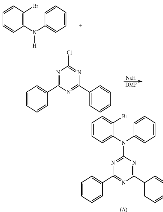
[Reaction Scheme 2]
