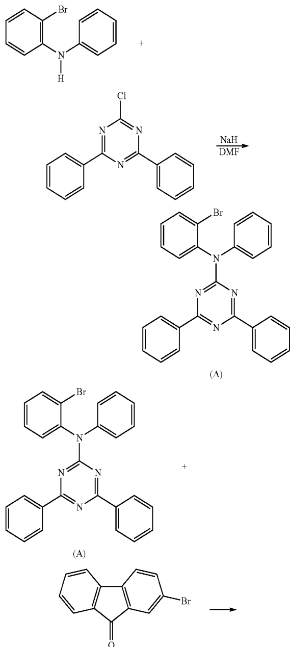
[Reaction Scheme 1]
