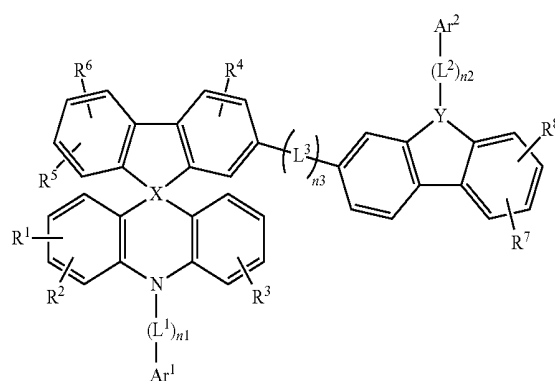
[Chemical Formula 2-3]
