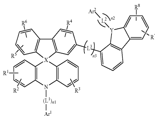
[Chemical Formula 2-3]
