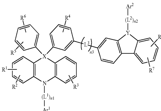
[Chemical Formula 1-2]
