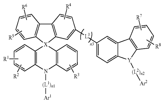
[Chemical Formula 2-1]
