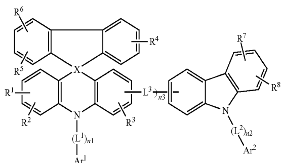
[Chemical Formula 4]
