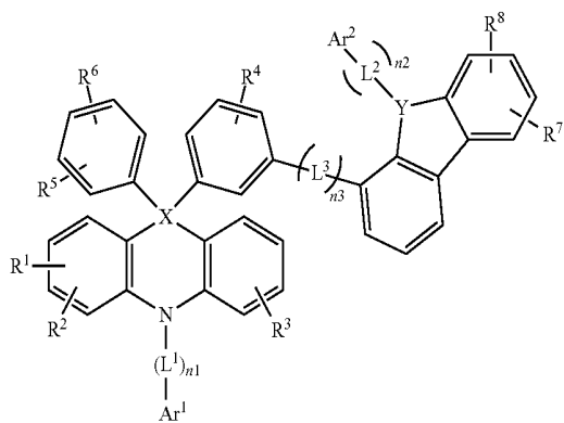
[Chemical Formula 1-3]
