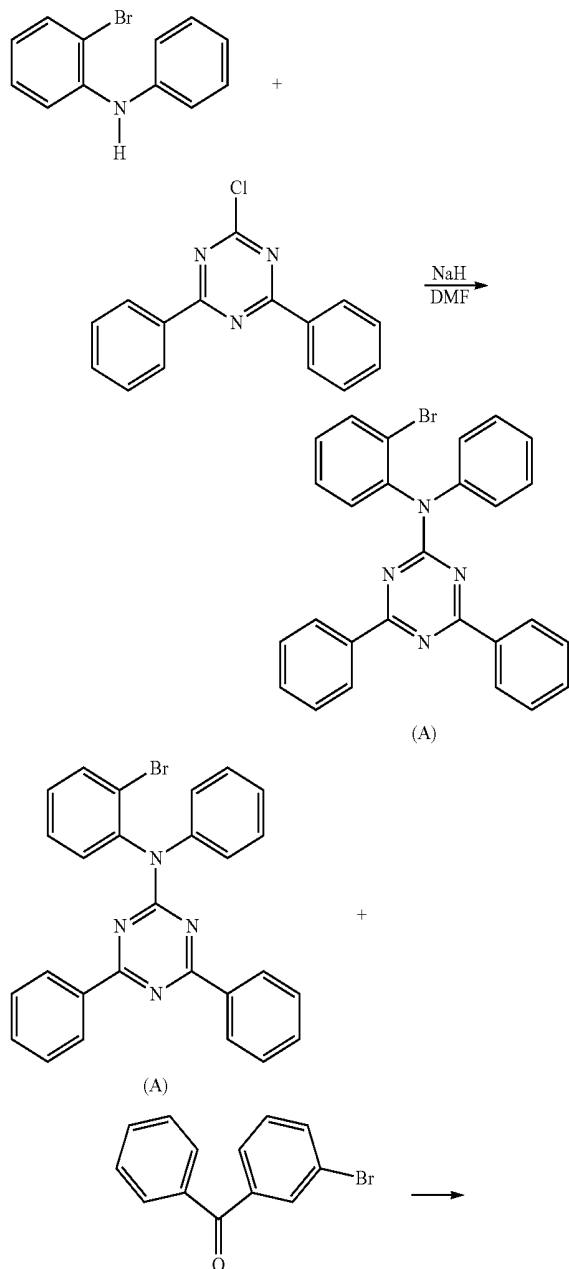
[Reaction Scheme 5]
