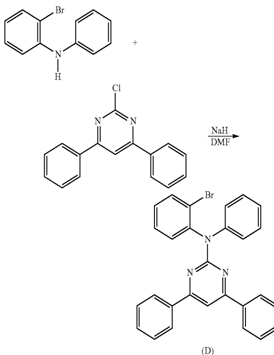
[Reaction Scheme 4]
