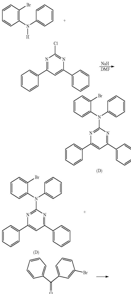
[Reaction Scheme 8]
