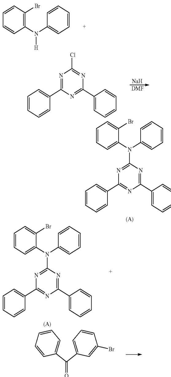
[Reaction Scheme 6]
