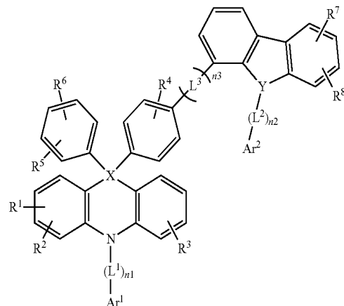
[Chemical Formula 2-1]
