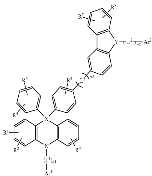
[Chemical Formula 1-5]
