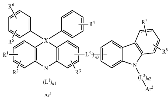
[Chemical Formula 3]
