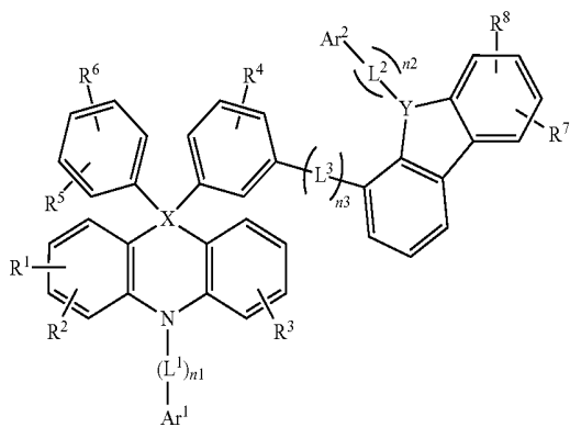
[Chemical Formula 1-4]
