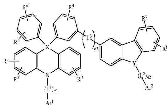
[Chemical Formula 1-2]
