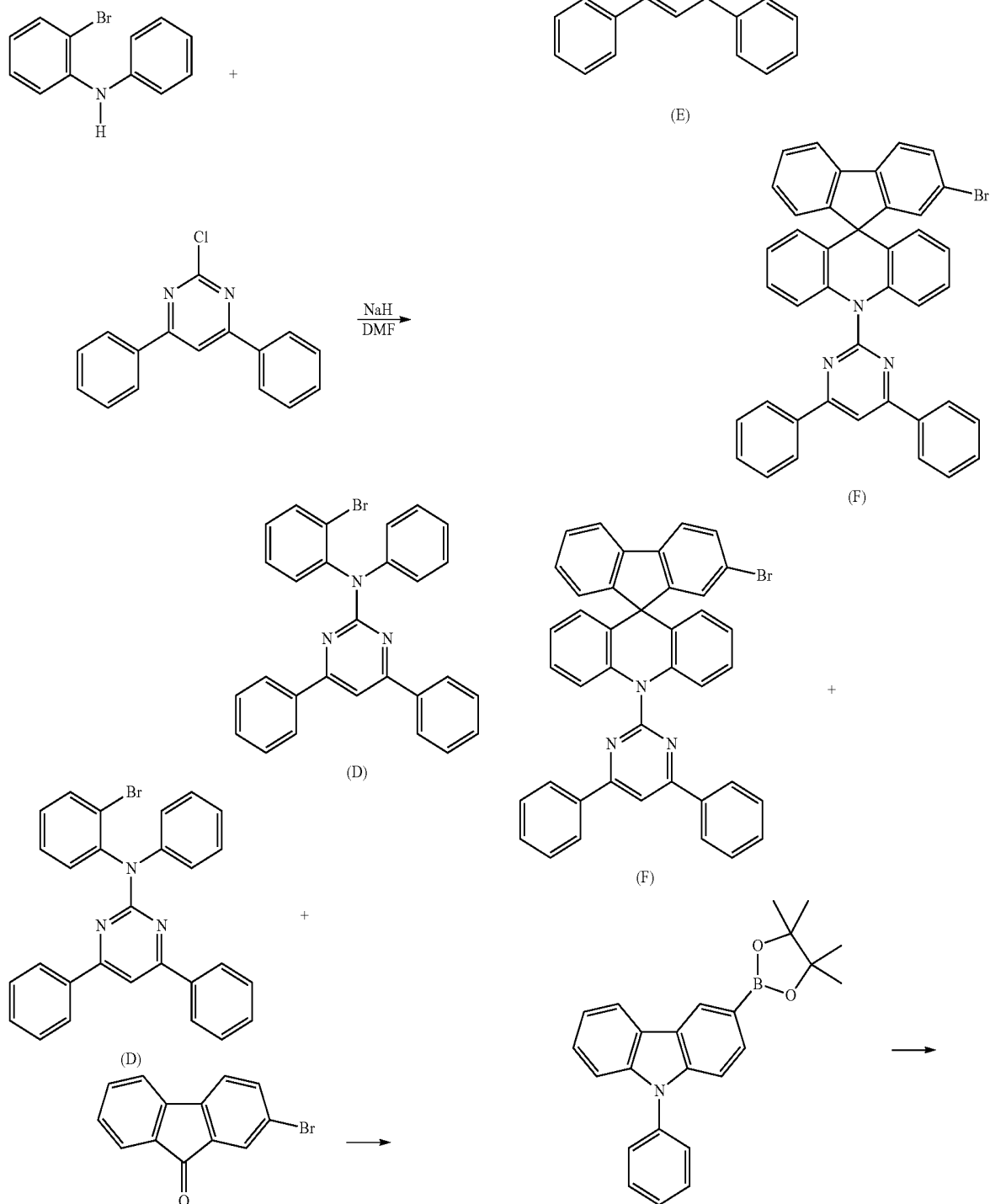
[Reaction Scheme 3]
