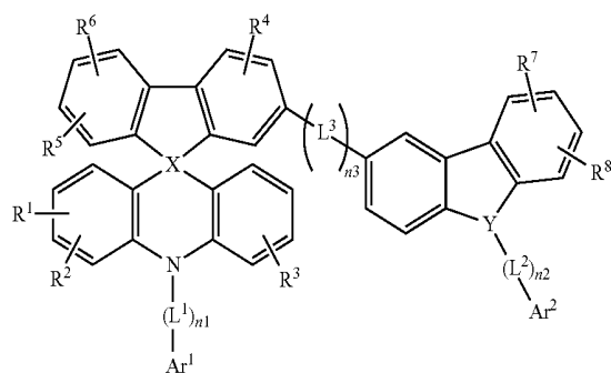
[Chemical Formula 2-2]
