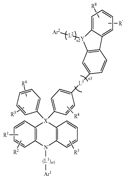
[Chemical Formula 1-5]
