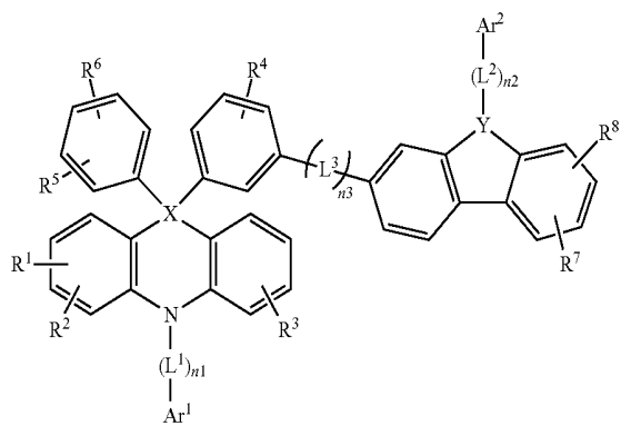
[Chemical Formula 1-2]
